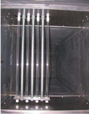
Figure 2-2. Device installed inside the test rig. There are 4 lamps and 3 support rods.
